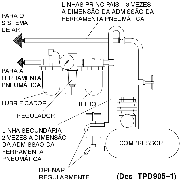
(Des. TPD905–1)
